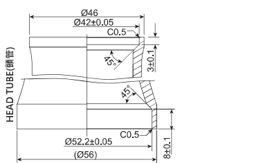
卡式下碗 STEEL LOWER CARTRIDGE CUP ④
