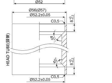
密封式軸承 A.C. SEALED BEARING ⑤
