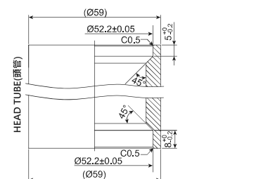
密封式軸承 A.C. SEALED BEARING ④
