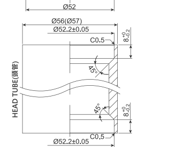
5 密封式軸承 A.C. SEALED BEARING
