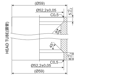
4 密封式軸承 A.C. SEALED BEARING
