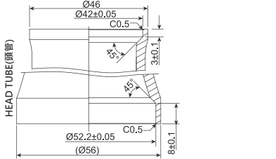
4 卡式下碗 STEEL LOWER CARTRIDGE CUP
